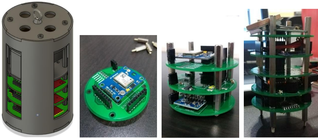
Views of Final Assembly of CanSat Built during above Workshops (Patents Filed)
