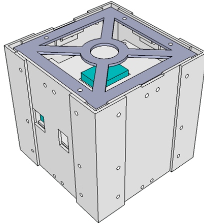
CSPDsatsat-1 [1U CubeSat Small Spacecraft of Serbia]
