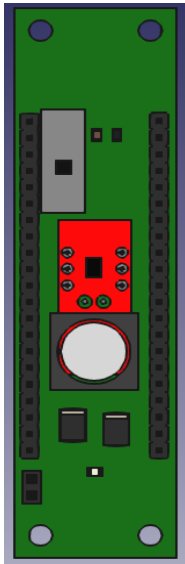
Top View Battery Board
